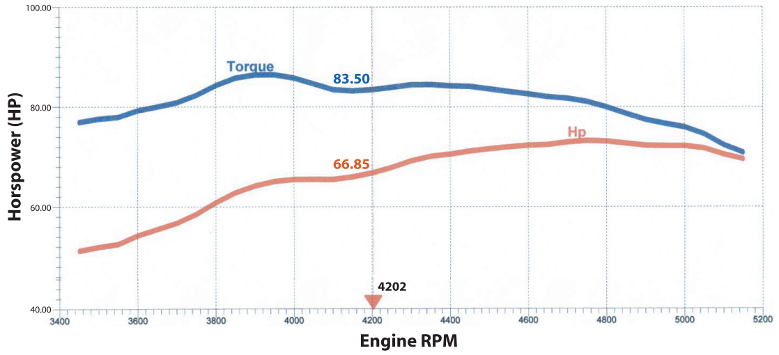
Peak Torque & HP vs. RPM
